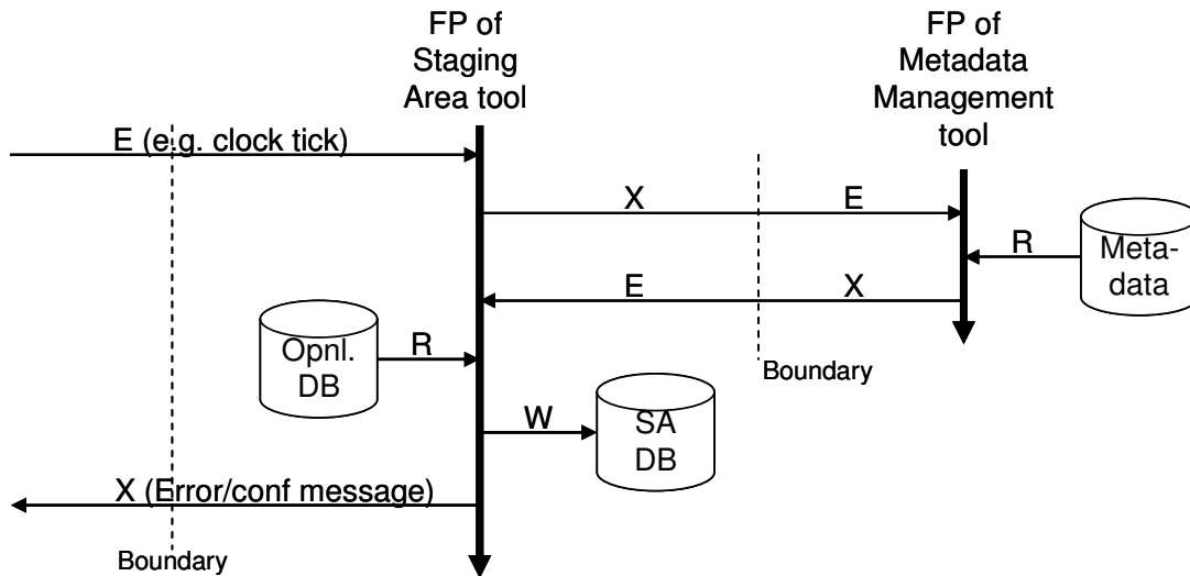
Figure 5: Interaction of the Staging Area tool and the Metadata Management tool
